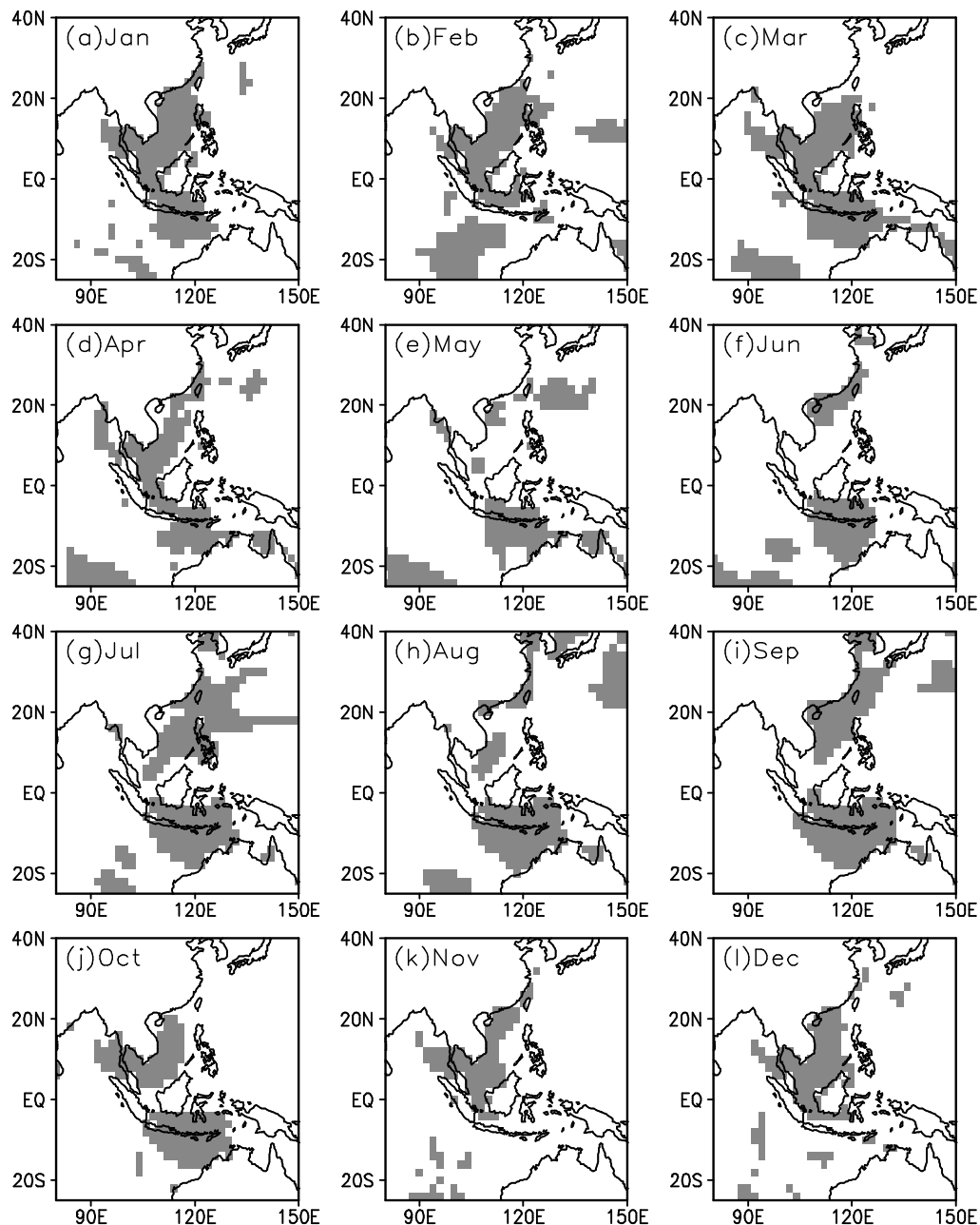
Fig. 1. Shading indicates where the SSTA lag correlation drops to the insignificant levels during October–December. (a)–(l) are for the starting months of January to December, respectively.
