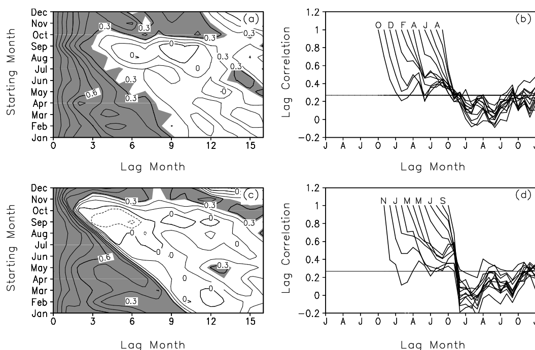
Fig. 8. Same as Figs. 2a–d, but for the “residual SSTA” in the SCS (upper panels) and the Indonesia region (bottom panels) obtained by subtracting the “ENSO-related SSTA” from the original SSTA in the SCS and the Indonesia region. The “ENSO-related SSTA” is formed by regressing the SCS and Indonesia SSTA upon the Niño-3 SSTA.
